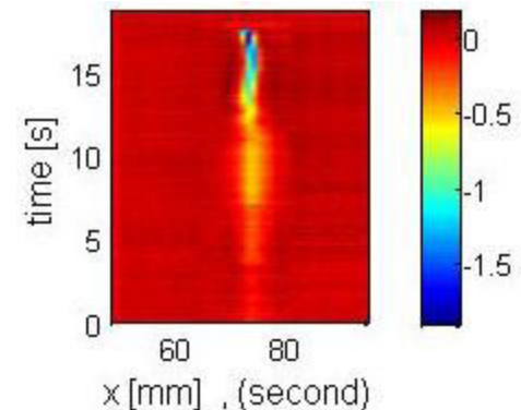
a-Carbon C-8
