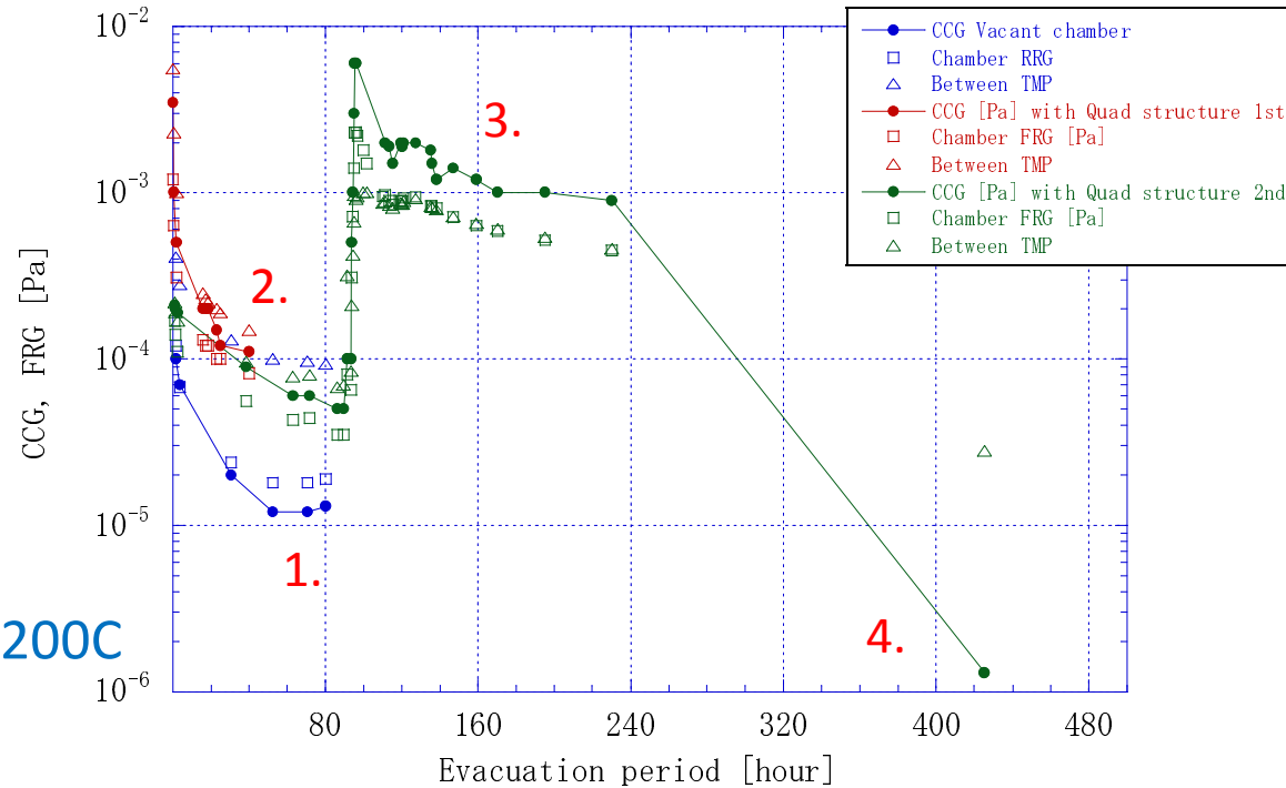
Chamber Evacuation
